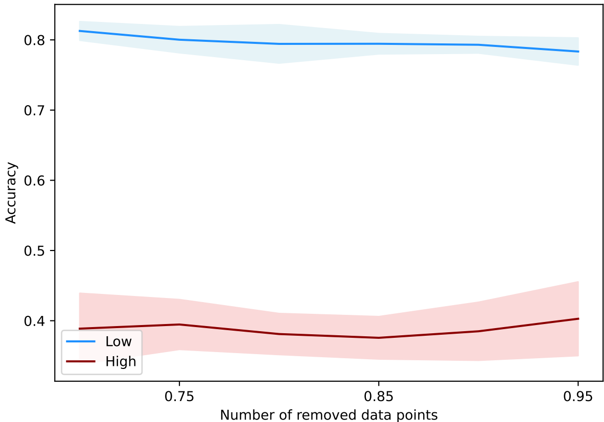
DataAttrOpt(10000, 0.03, 15, best, +b, alpha=best) - imdb-embedding
